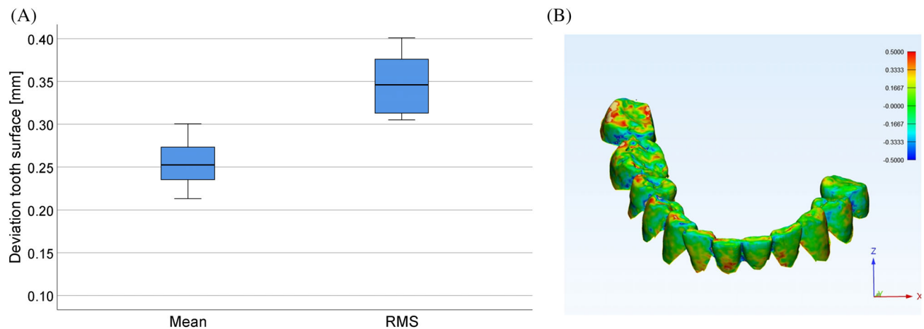
FIGURE 5 Geometric deviations of occlusal surfaces between model scans and MRI-derived occlusal reconstructions. A, Boxplots of mean value (left) 0.254 \text{ mm} \pm 0.026 \text{ mm} and root mean square (RMS) value (right) 0.347 \pm 0.034 \text{ mm} . B, Color mapping showing distribution of geometric deviations (limits set from -0.5 to +0.5 mm) of a MRI-derived occlusal reconstruction compared to occlusal surface of corresponding model scan in a sample patient
