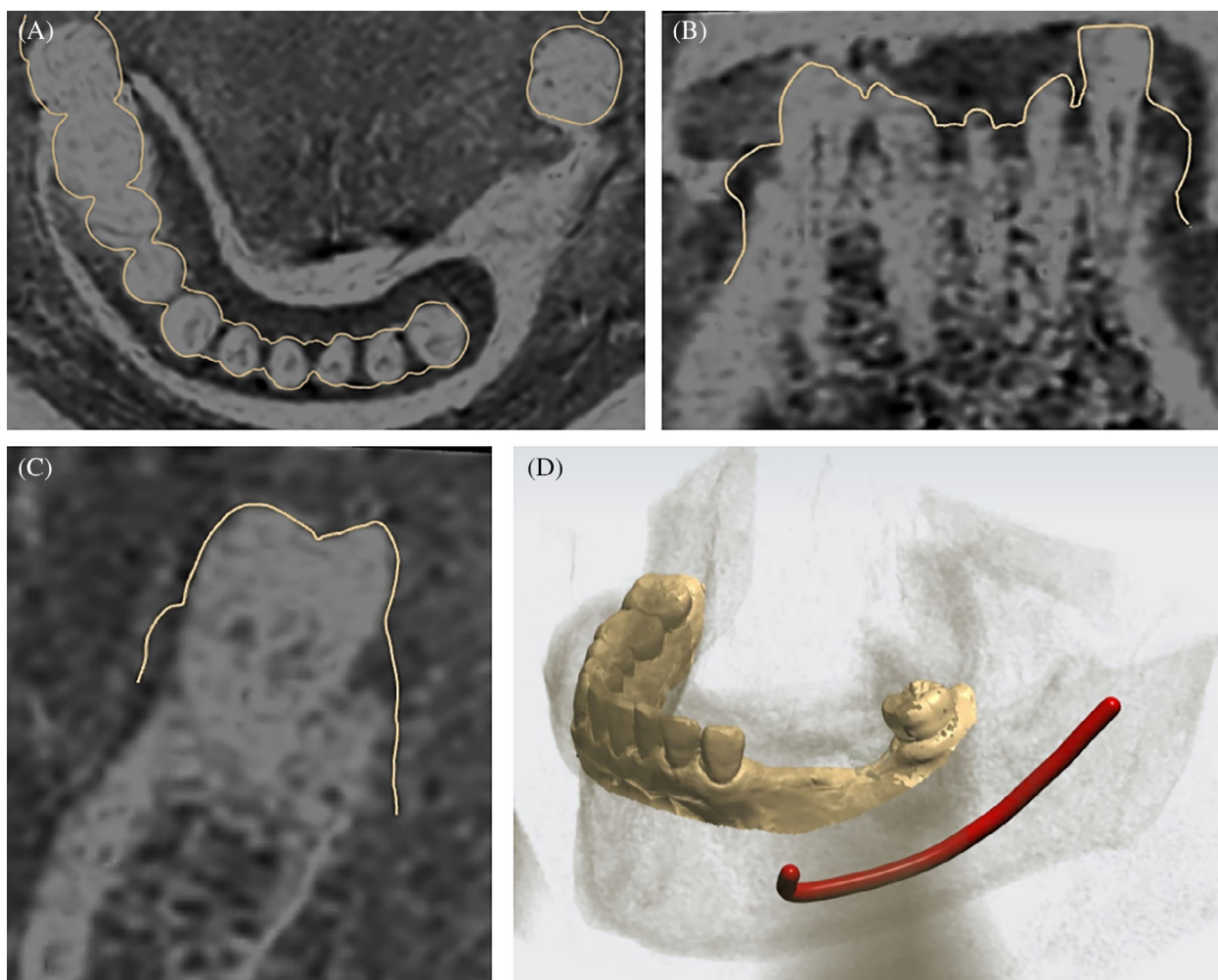
FIGURE 1 Top and Bottom left: Digitalized occlusal surfaces derived from a model scan (beige lines) are superimposed with MRI DICOM data in the planning software. The alignment is fine-tuned in the coronal, axial and sagittal planes using translation and rotation tools to achieve an exact matching. Please note: In this case, the signal values of the T1-weighted images were previously inverted (black to white) to provide a CBCT-like appearance. Bottom right: Resulting 3D “Hybrid Model” with the traced inferior alveolar nerve (displayed in red)
